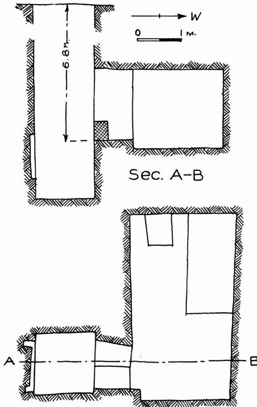
52. G 7111 A, plan and section
