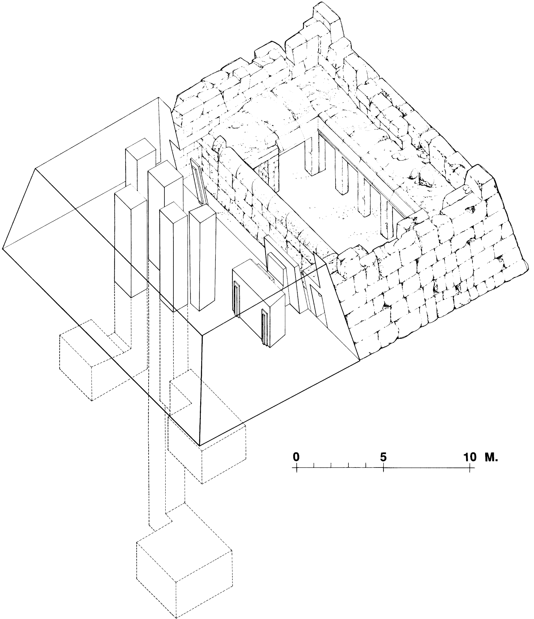
5. Axonometric drawing of tomb G 6040, showing the position of shafts and burial chambers. Re-surveyed and drawn by Charles V. Belson
