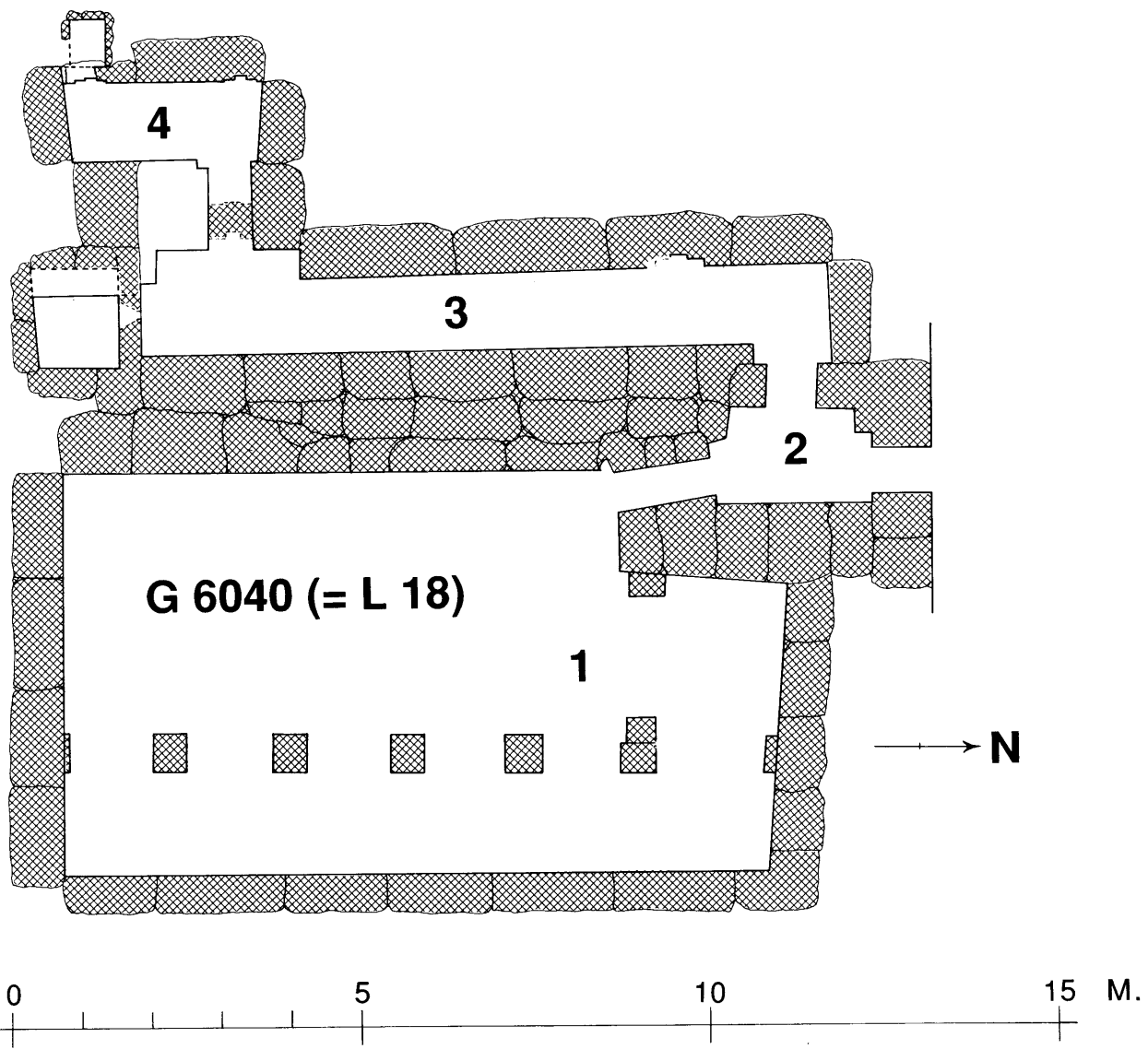
8. General plan of G 6040 showing chamber designations. Drawn by A. Floroff
