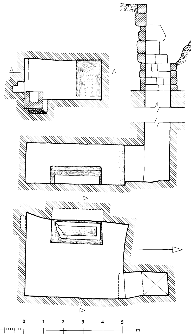
68. G 6020, shaft A: Plan and sections
