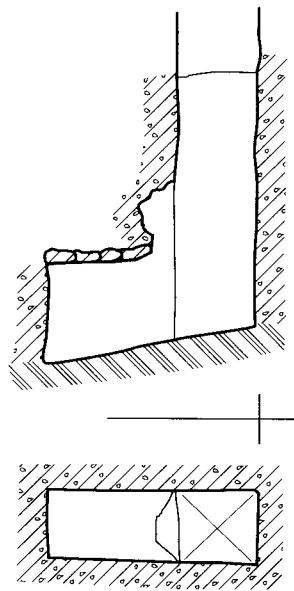
101. G 6034, shaft R: Plan and section
