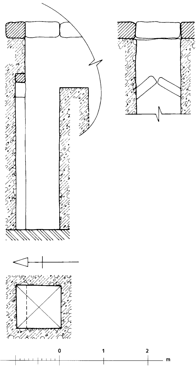
107. G 6040, shaft A: Plan and sections
