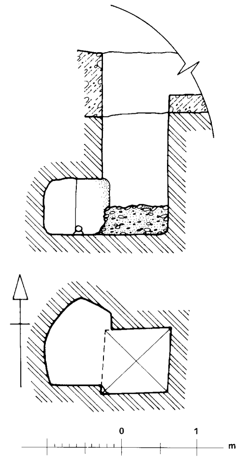
117. G 6041, shaft X: Plan and section
