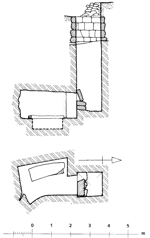
119. G 6042, shaft A: Plan and section
