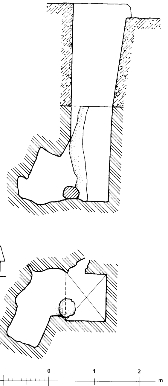
69. G 6021, shaft A: Plan and section
