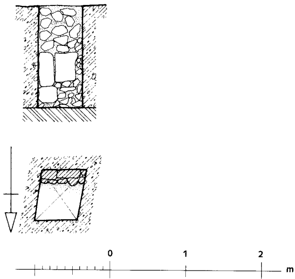
67. G 6014, shaft E: Plan and section
