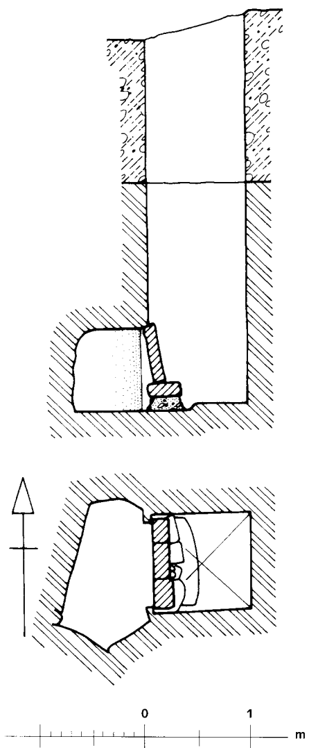
116. G 6041, shaft F: Plan and section
