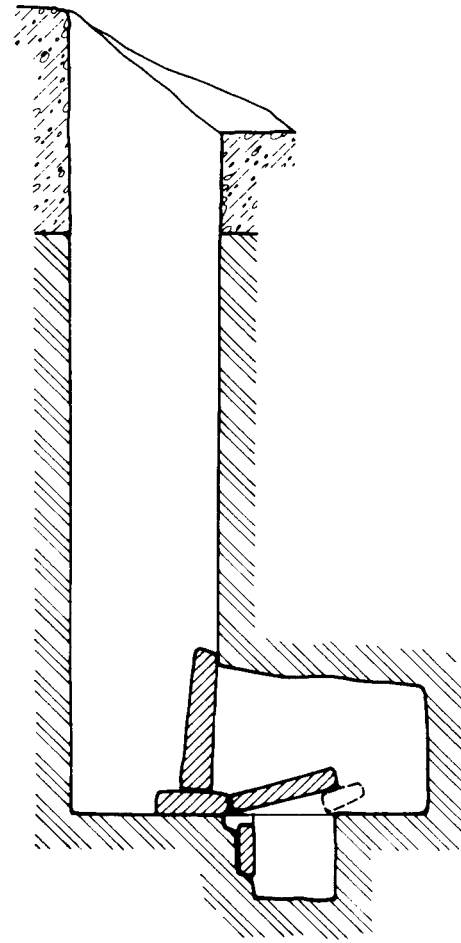
60. G 6012, shafts A and B: Plans and sections
