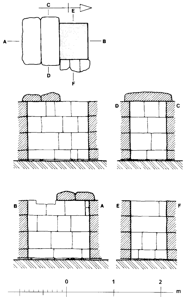
118. G 6042: Plan and sections of serdab
