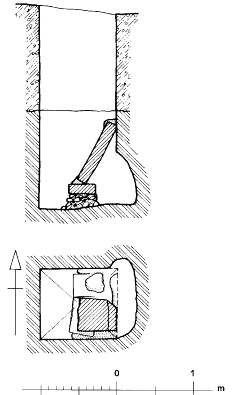
115. G 6041, shaft E: Plan and section
