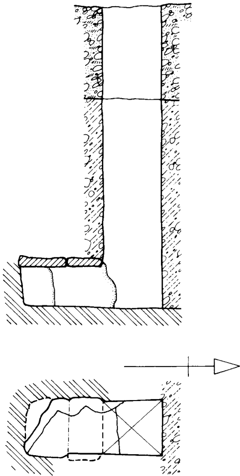
94. G 6034, shaft K: Plan and section
