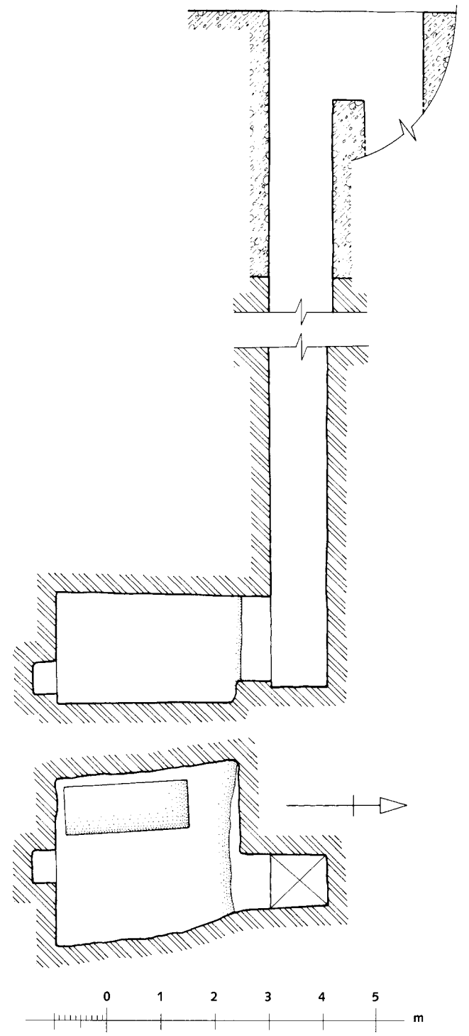
108. G 6040, shaft B: Plan and section
