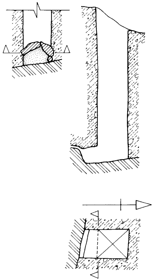
93. G 6034, shaft I: Plan and sections
