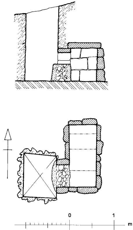
114. G 6041, shaft D: Plan and section
