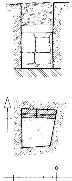
65. G 6014, shaft C: Plan and section of burial
