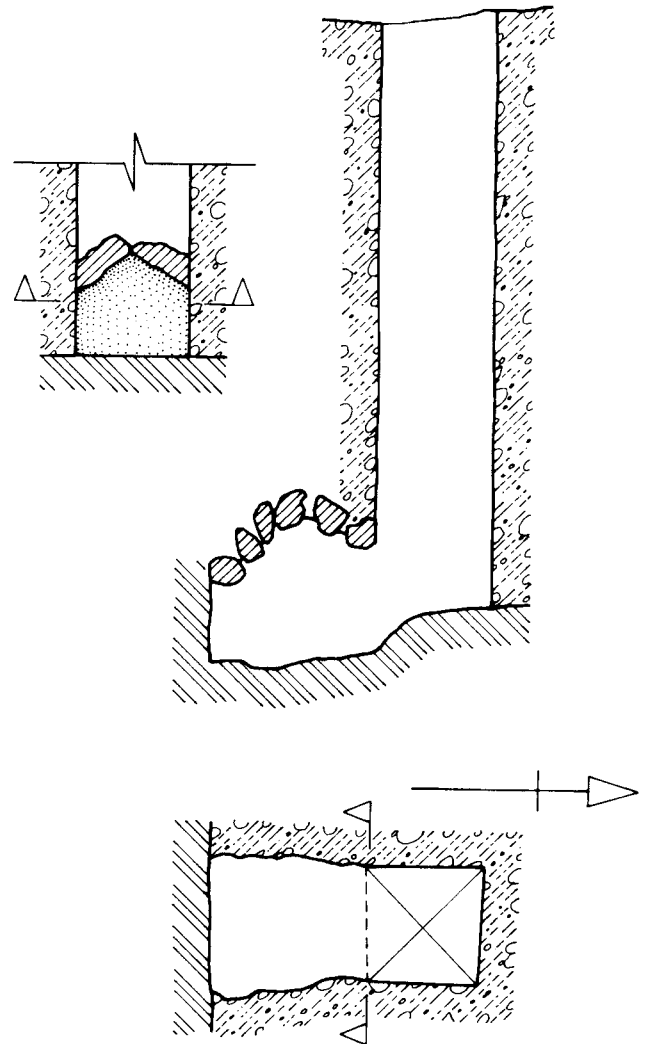
95. G 6034, shaft L: Plan and sections
