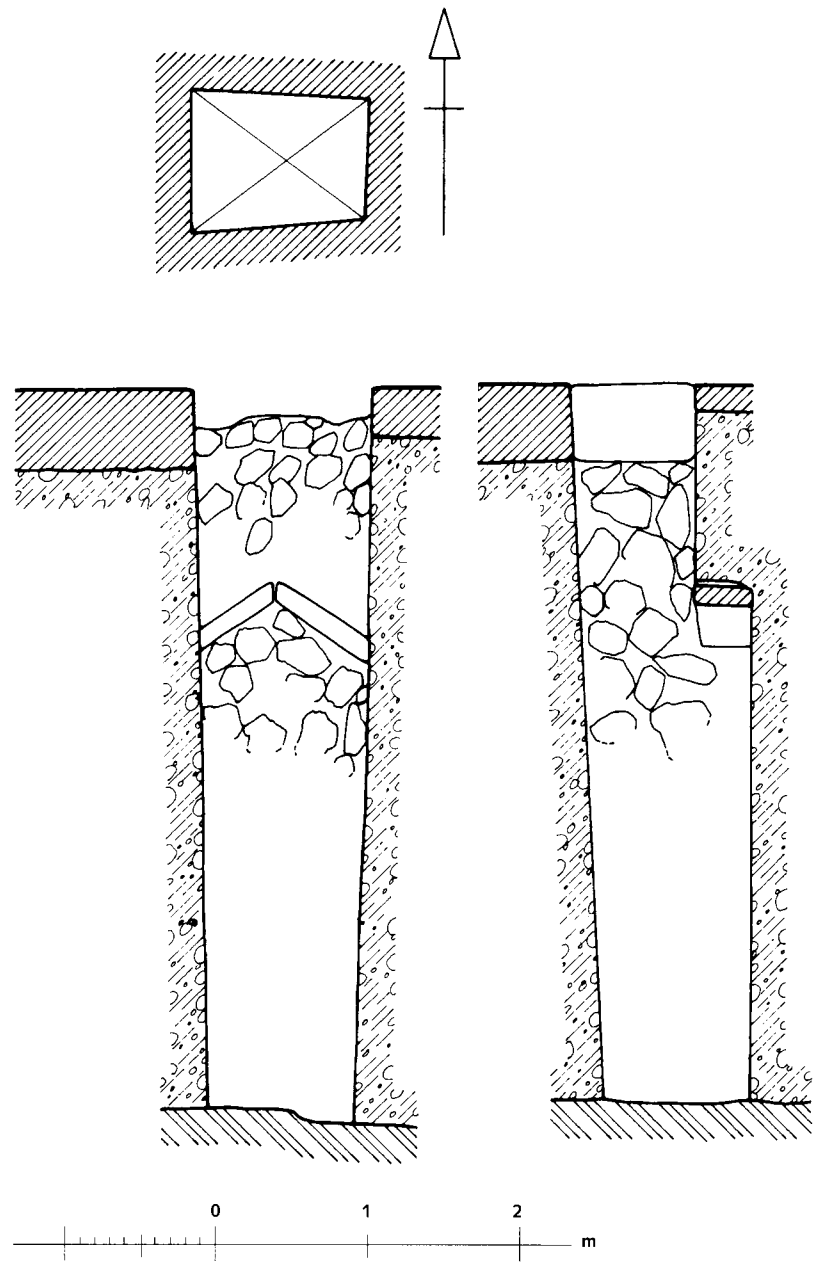
110. G 6040, shaft C: Plan and sections
