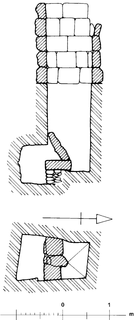
120. G 6042, shaft B: Plan and section
