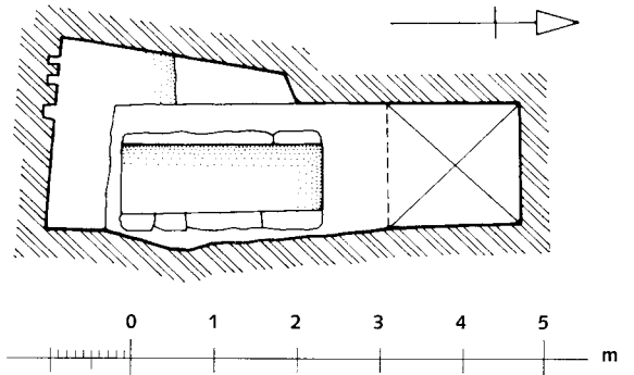
125. G 6050, shaft A: Plan and section
