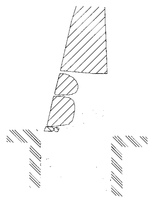
79. G 6030, shaft B: East-west section of burial chamber
