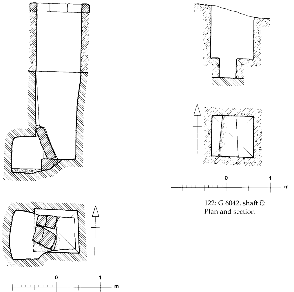
121. G 6042, shaft D: Plan and section
