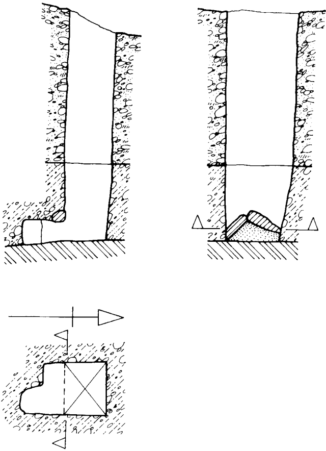
91. G 6034, shaft G: Plan and sections
